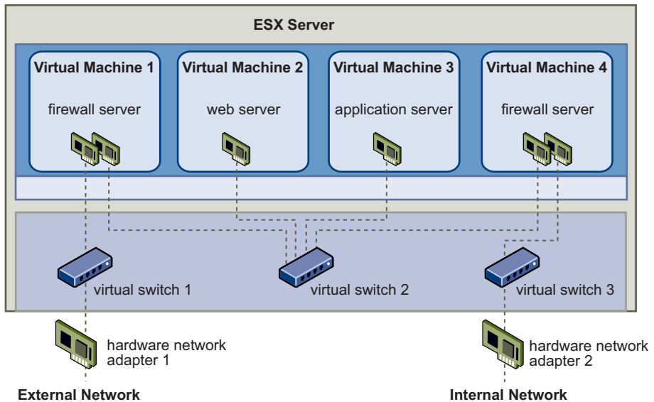
Figure 9-4. DMZ Configured On a Single ESX Server Host
