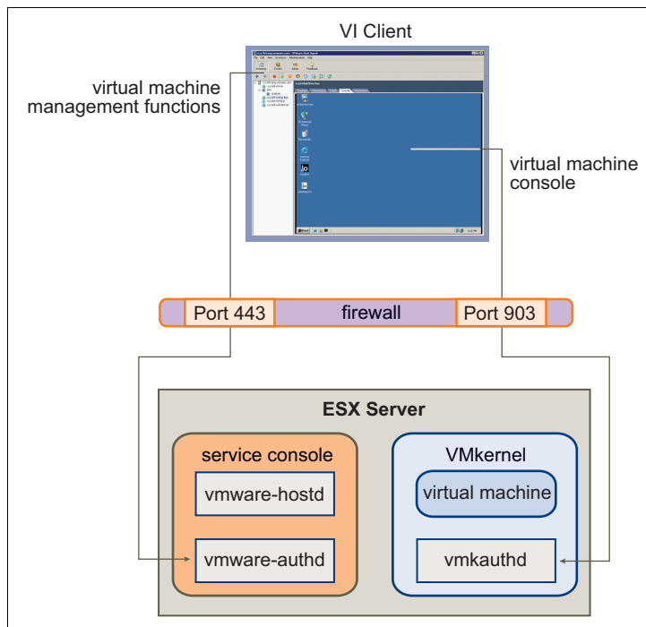
Figure 10-3. Port Usage for VI Client Communications with ESX Server 3
