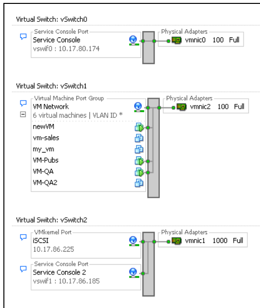
Figure 10-5. iSCSI Storage on a Separate Virtual Switch
