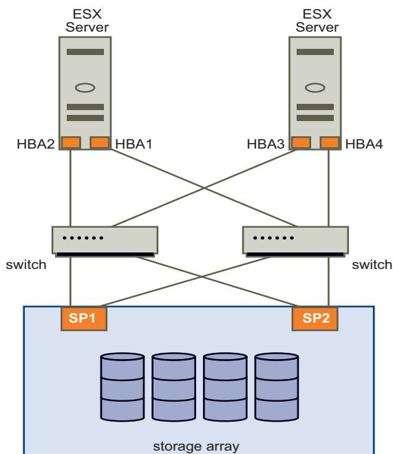
Figure 7-1. Fibre Channel Multipathing
