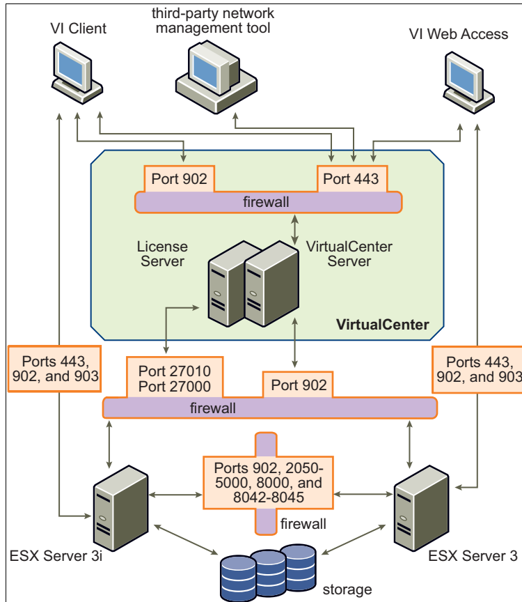
Figure 10-1. Sample Virtual Infrastructure Network Configuration and Traffic Flow
