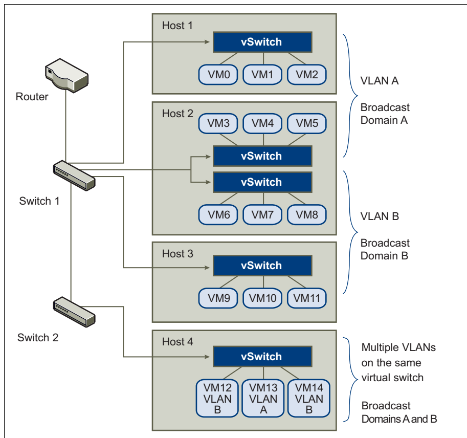
Figure 10-4. Sample VLAN Layout
