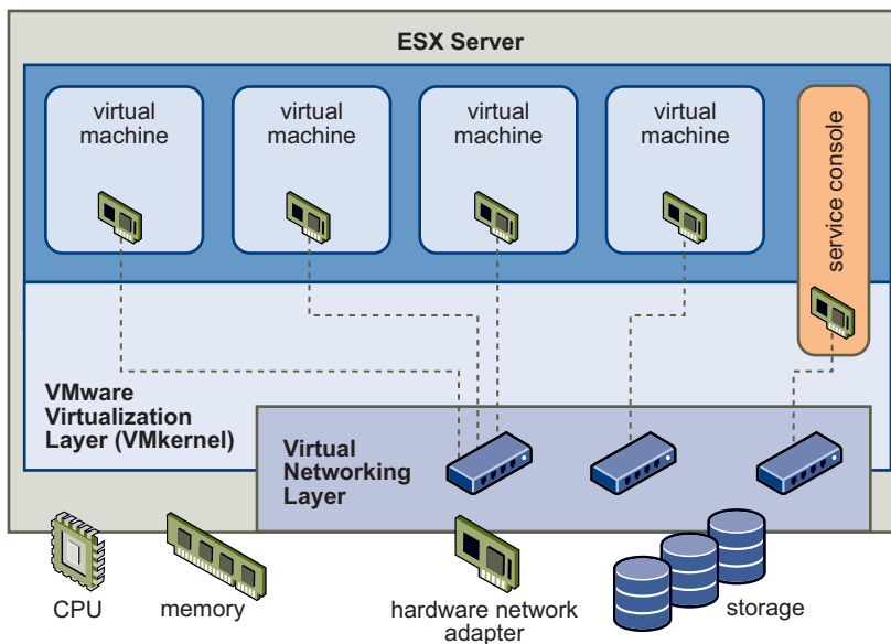
Figure 9-1. ESX Server 3 Architecture
