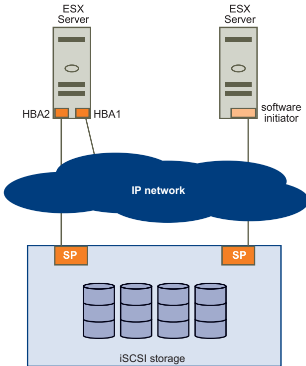
Figure 7-2. iSCSI Multipathing
