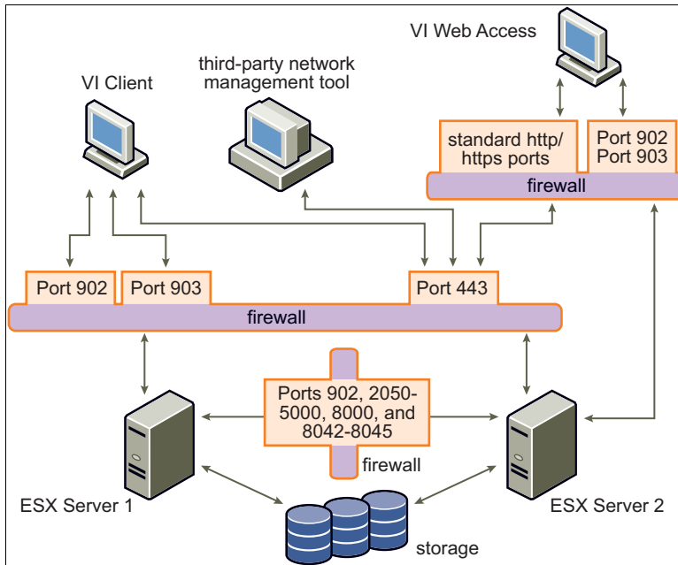
Figure 10-2. Firewall Configuration for ESX Server 3 Networks that a Client Manages Directly
